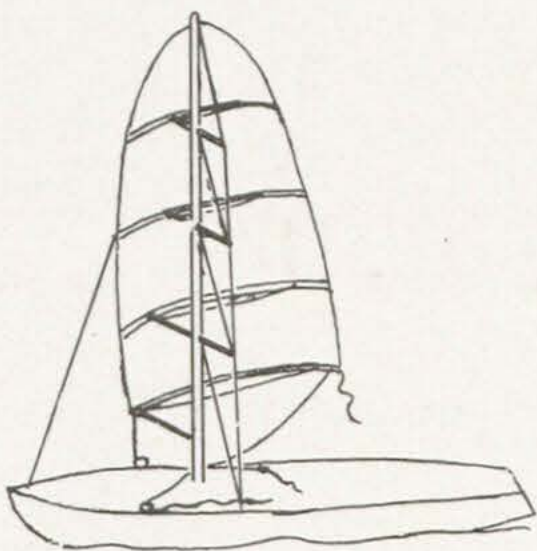
Fig. 9. Outside the shrouds square lugsail. Sprits slide in mast groove. Port shrouds only shown.
