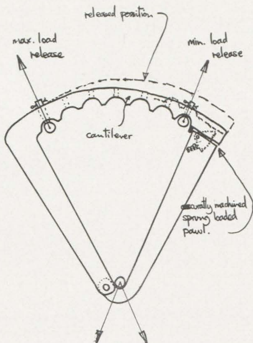
R. L. Cundall's Weak Link System.
