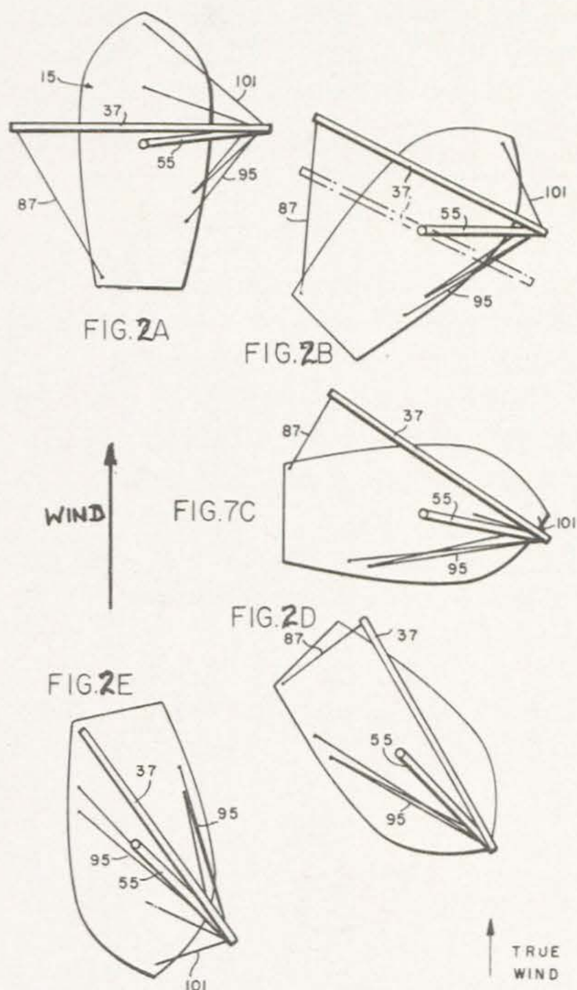
E. F. Hiscock's rig: position of spars on various courses.
