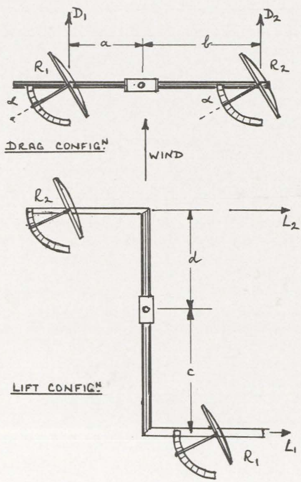
J. Norwood's Sail-Rig Comparison proposal
