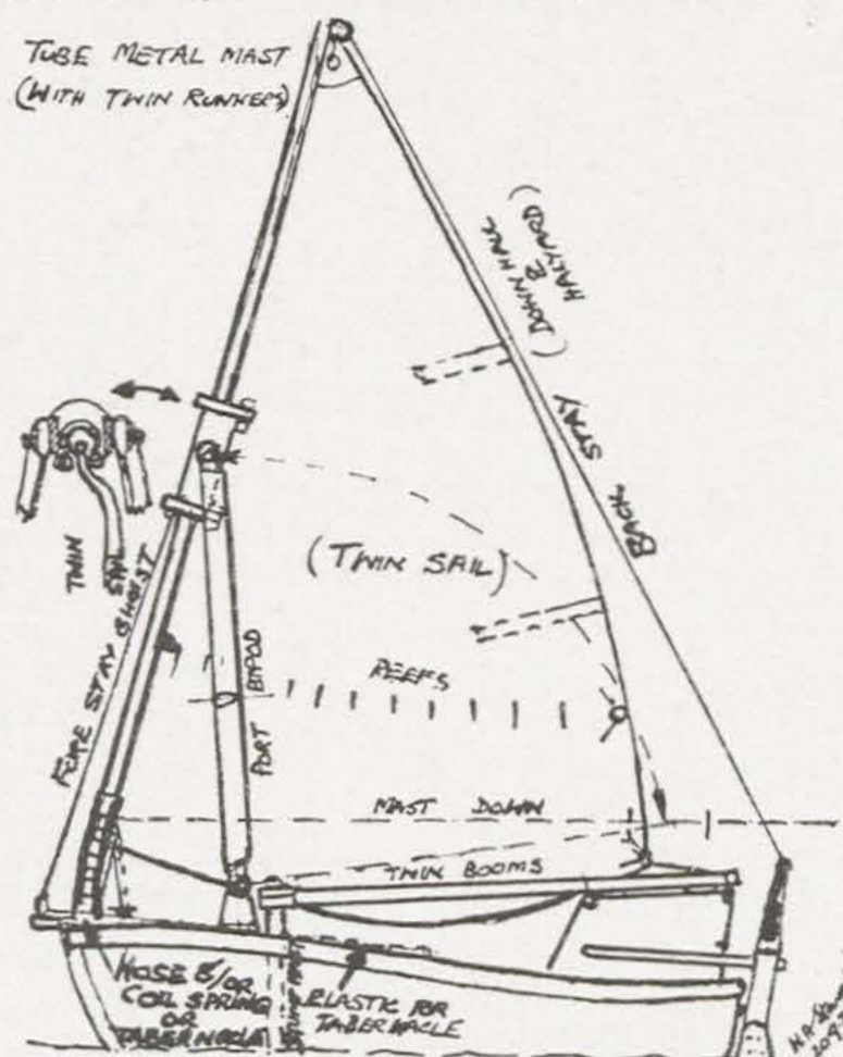
W. A. Stewart's Folding Bipod Lateen.
