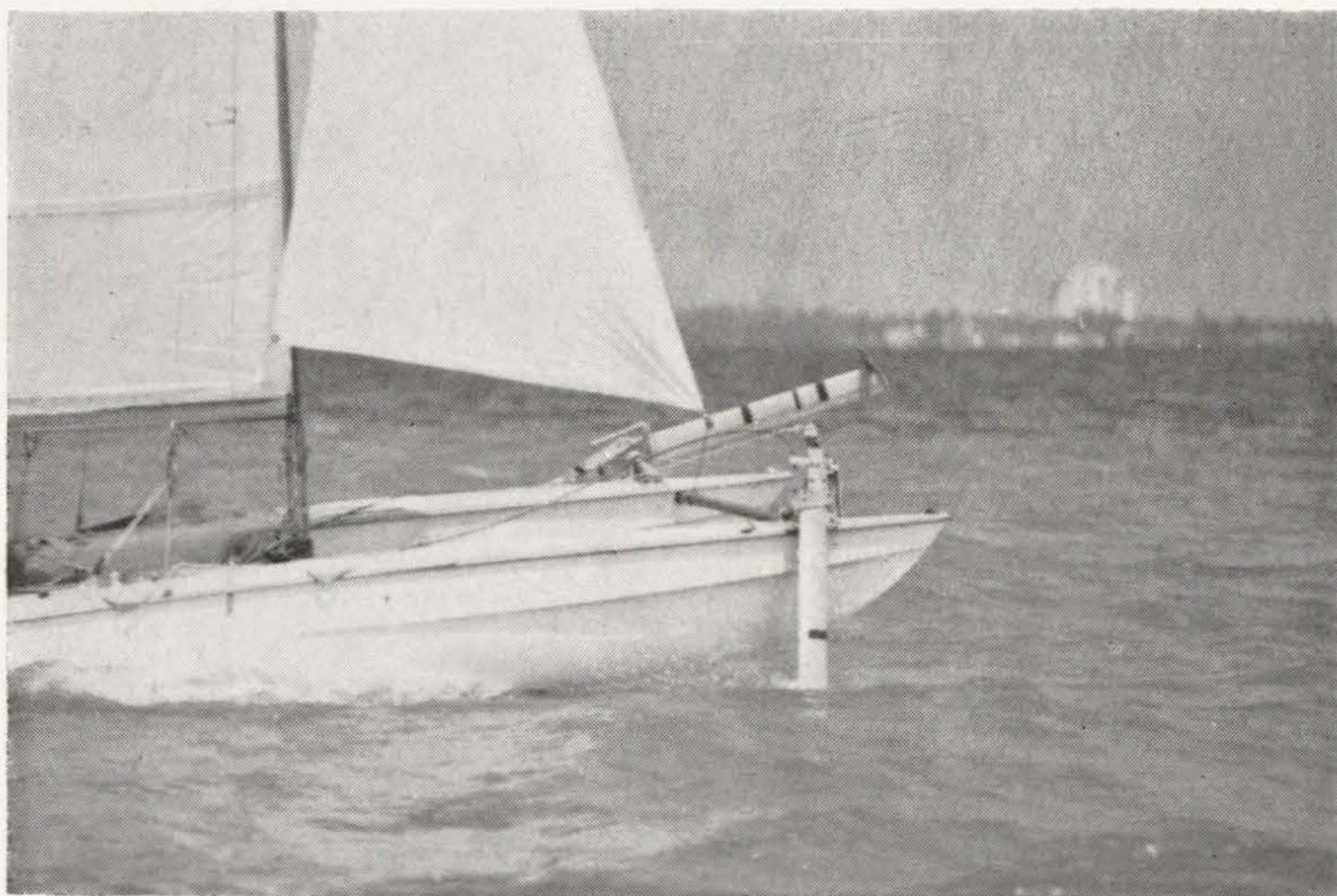
The Williams foil lifting the lee bow
