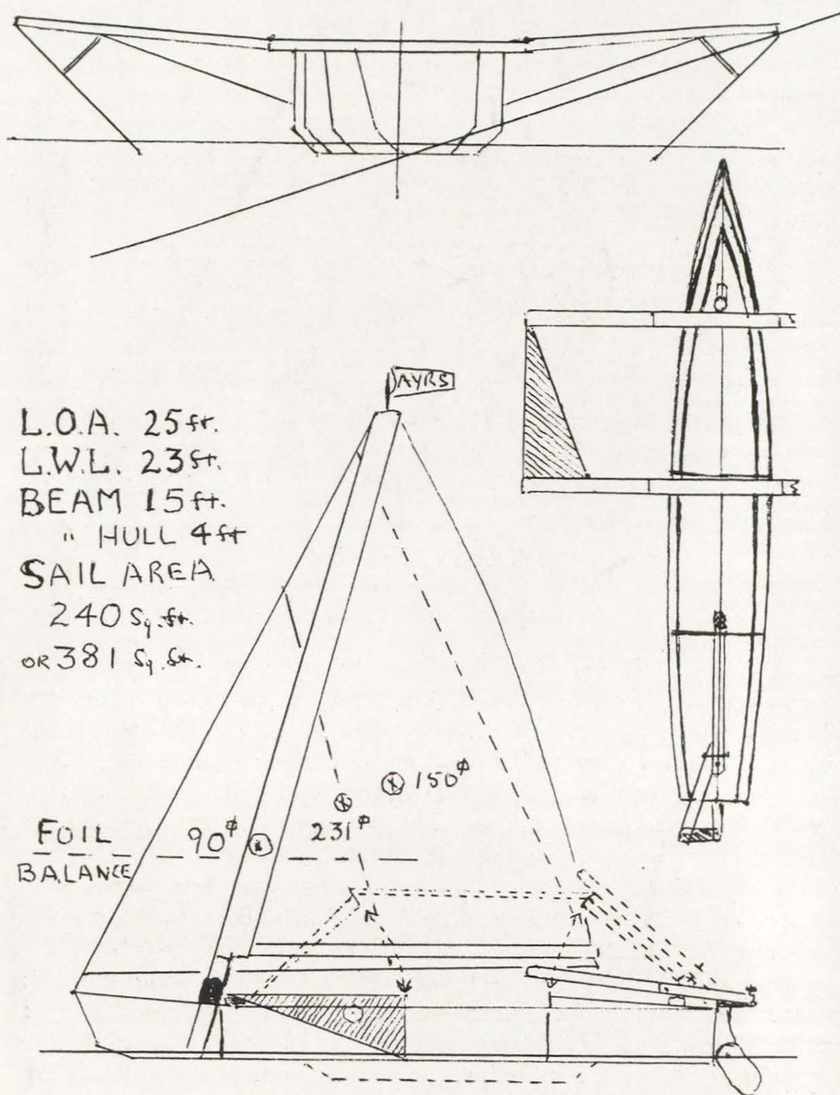
The Kinnegoe Cruiser
