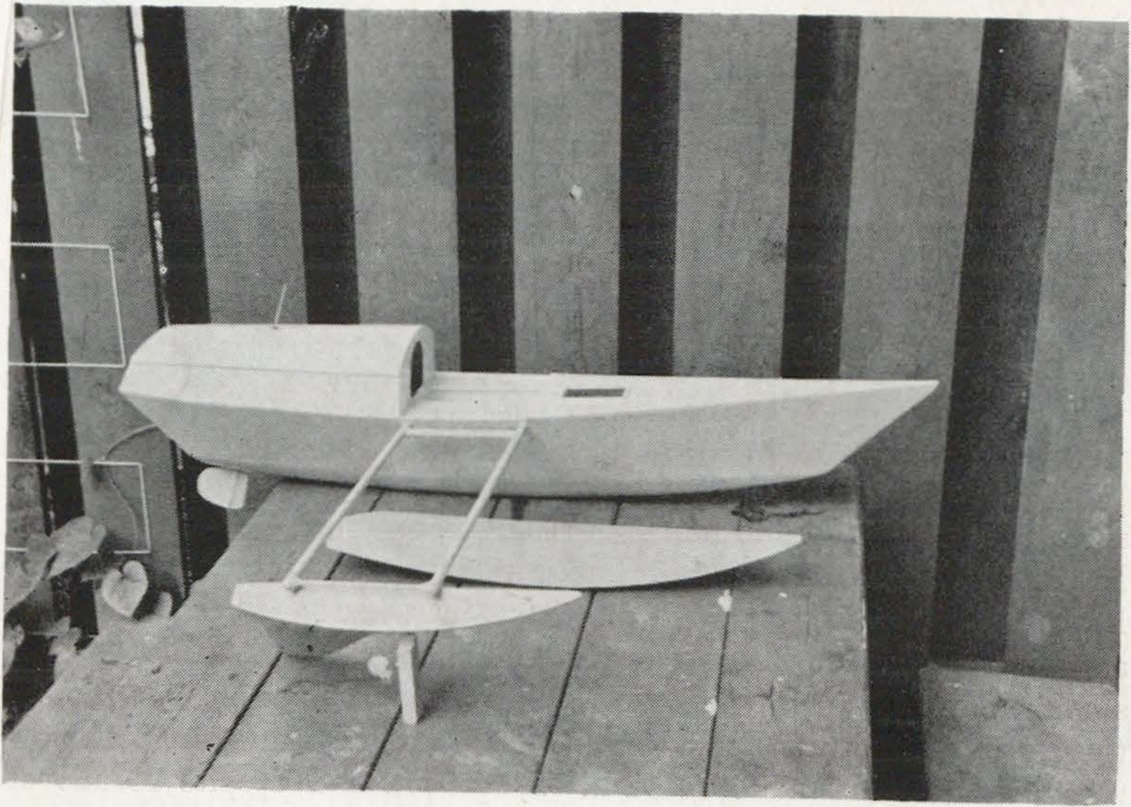
Bob Perkins' model foil cruiser
