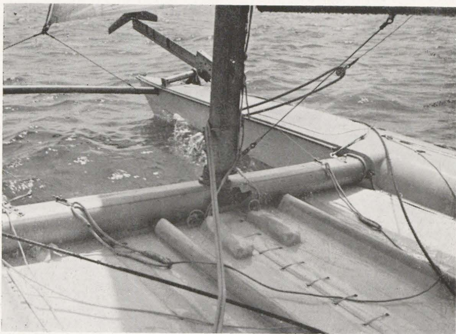
William's foil, retracted
