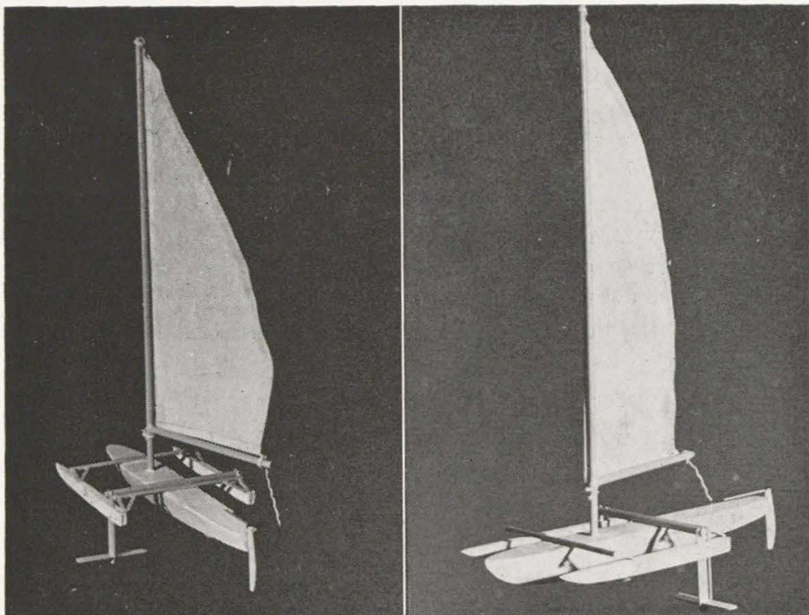
The Nason foil model
