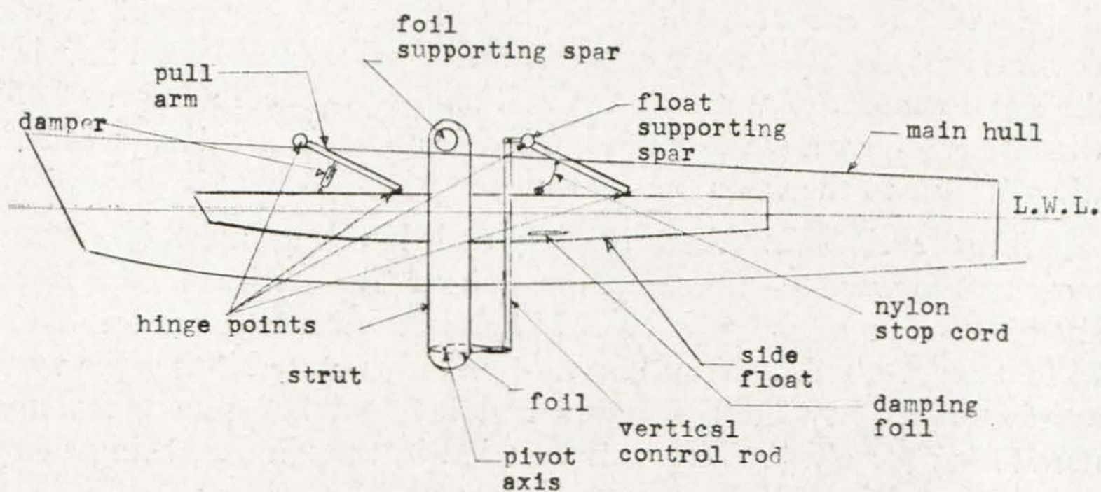
Figure 1.- General arrangement of parts
