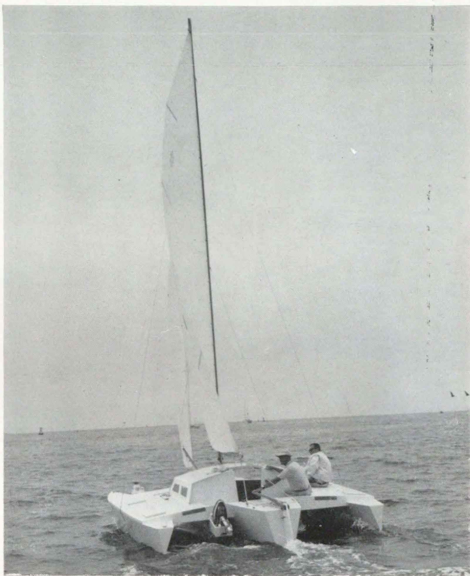
24 foot Cross trimaran.
