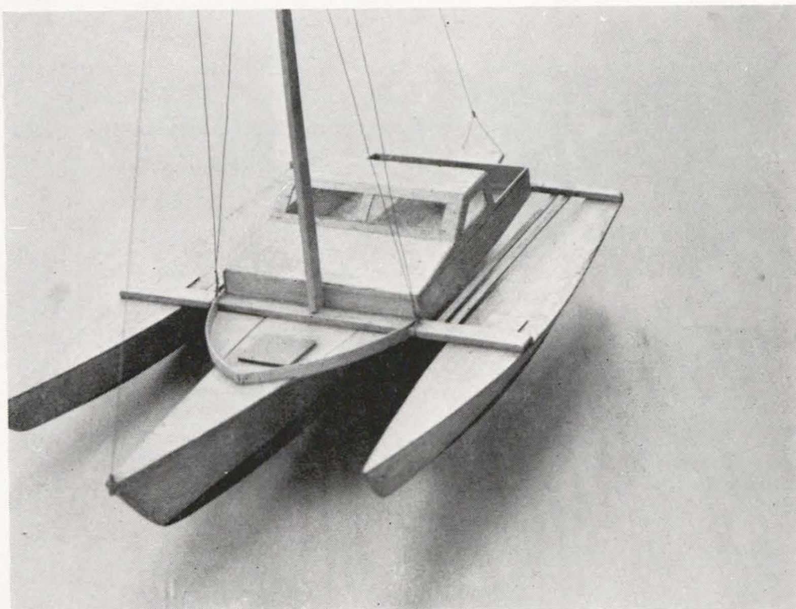
Model of 24 foot Trimaran.
