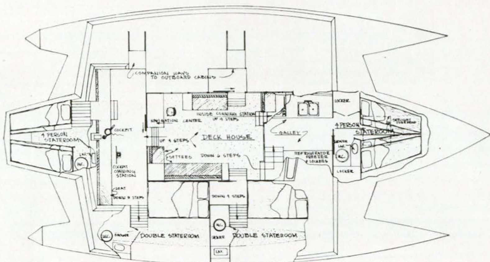
ACCOMMODATION PLAN
