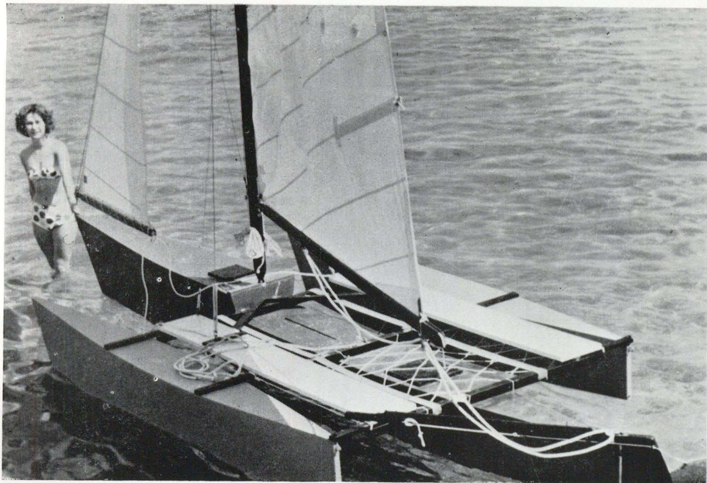
Trimaran with Quickcat main hull.
