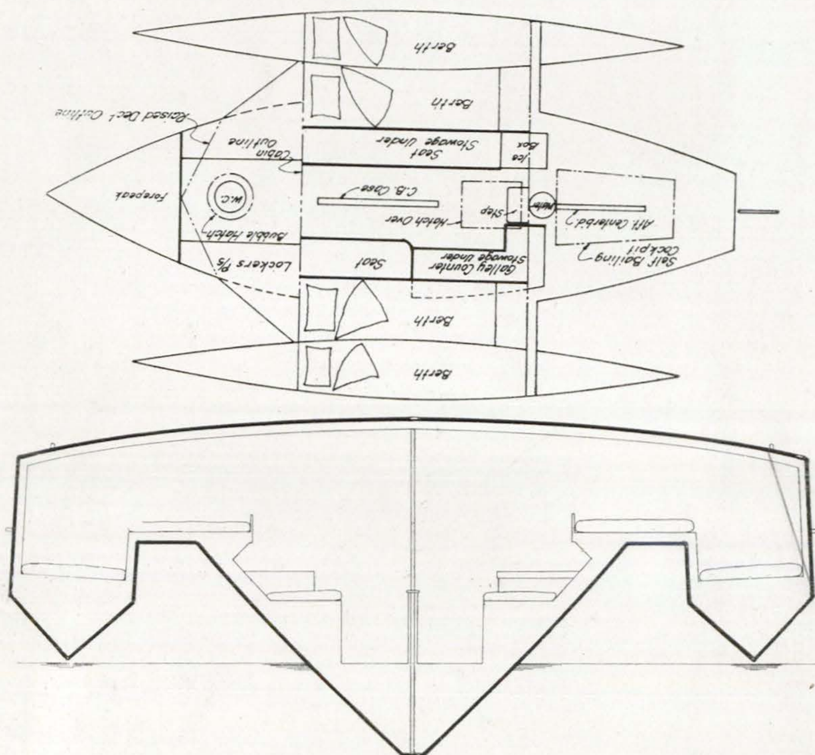
TRIDENT—Hull section and plan.
