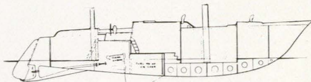
ELEVATION ON S. OF MAIN HULL
